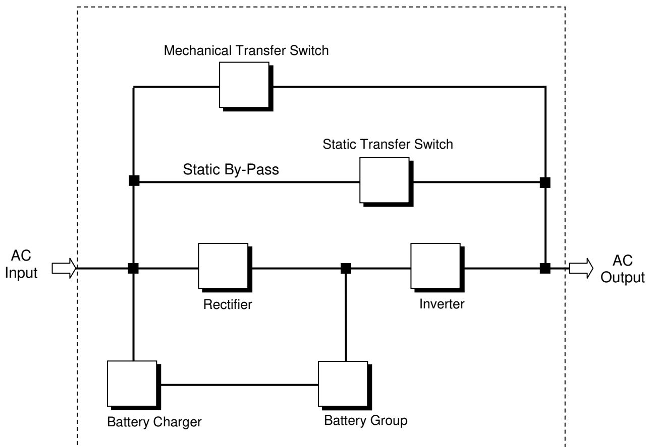
Figure 2.1 UPS Block Diagram
